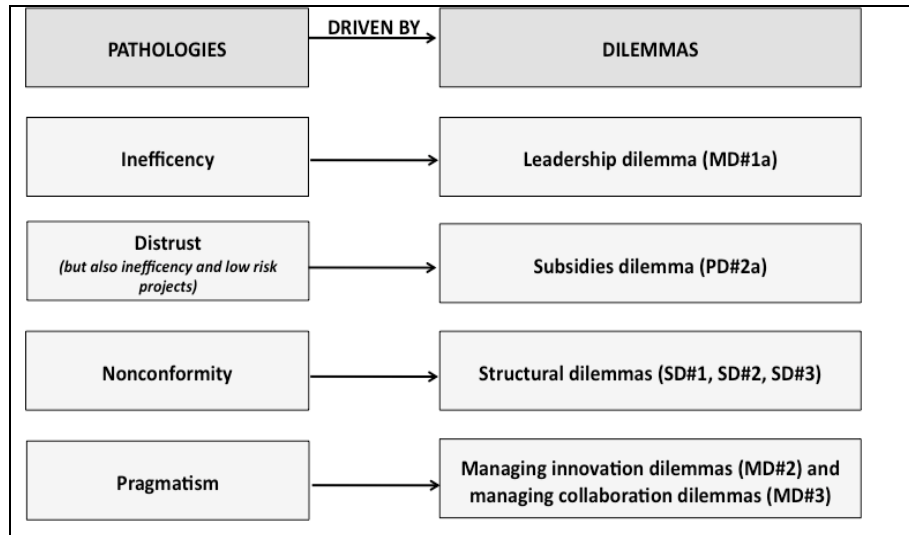
Figure 48: Summary of identified pathologies driven by associated dilemmas
